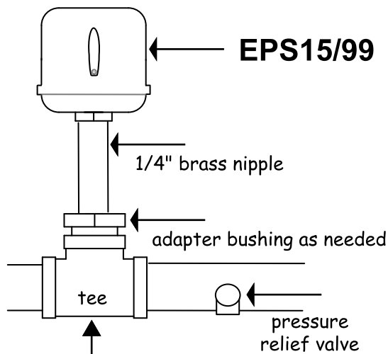
Typical installation
